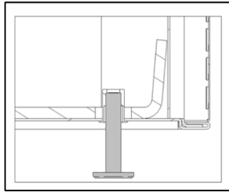
Illustration 8 : Pattes ajustables
