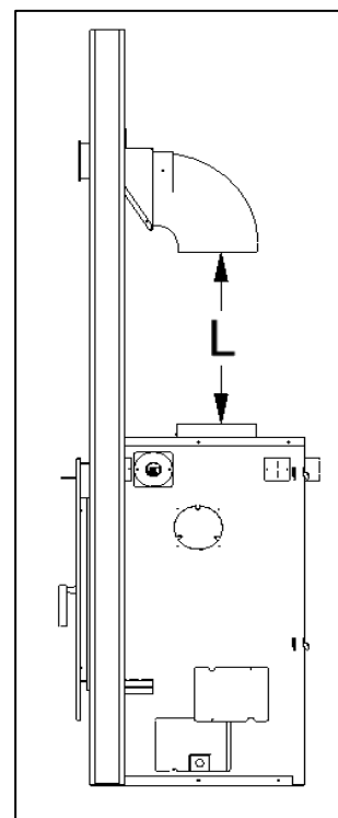
Illustration 3-27 : Distance L
